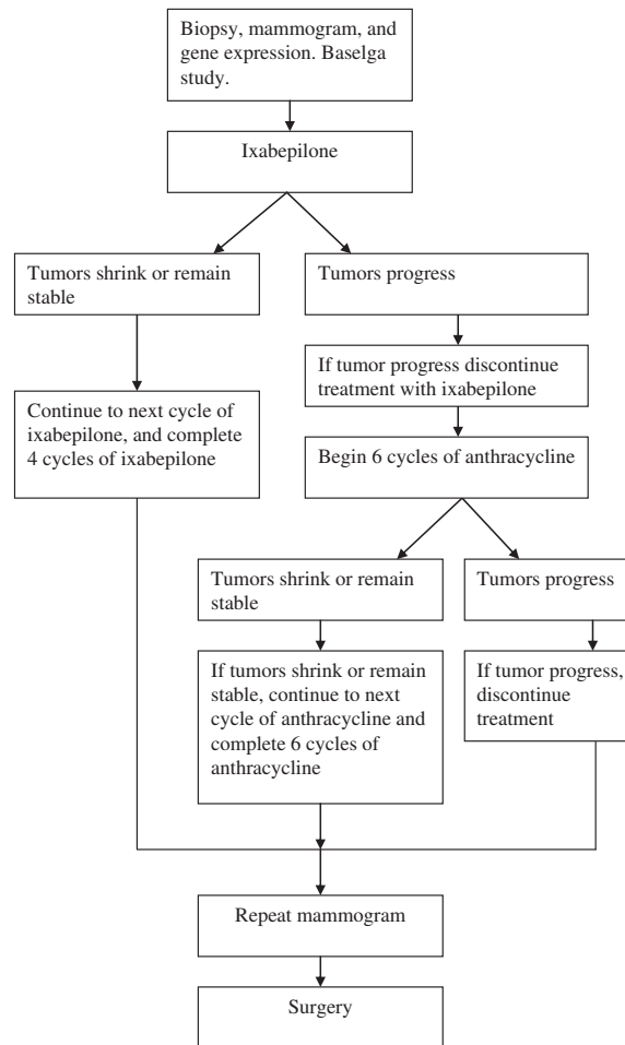
FIGURE 2.12 Schema with boxes showing decision points. Forked arrows indicate time points when tumors were assessed, and when a decision was made to proceed with the indicated course of action.
