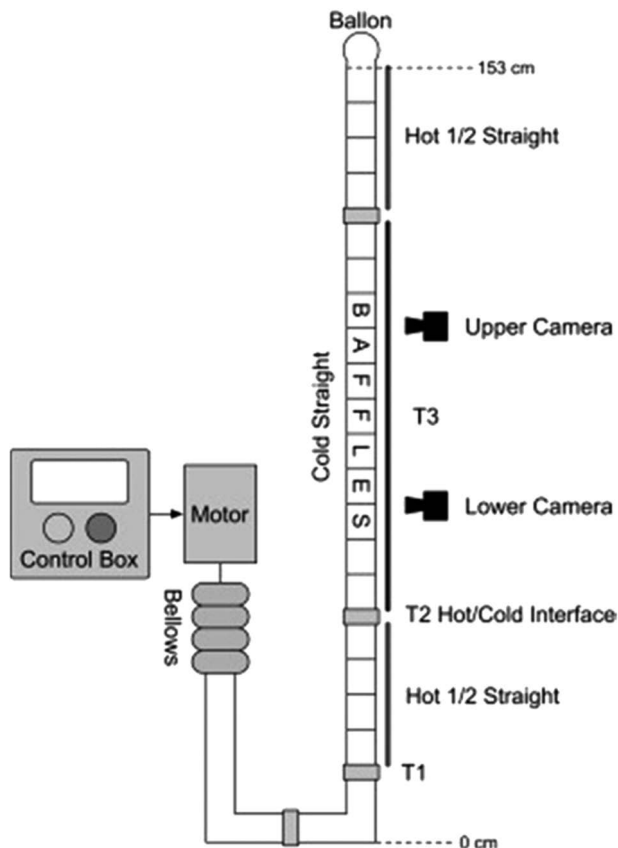
Figure 9.9 Experimental setup showing positions of temperature measurement, cameras, glass sections and collars which connect the glass components together. 31 Reproduced from ref. 31 with permission from Elsevier, Copyright 2015.
