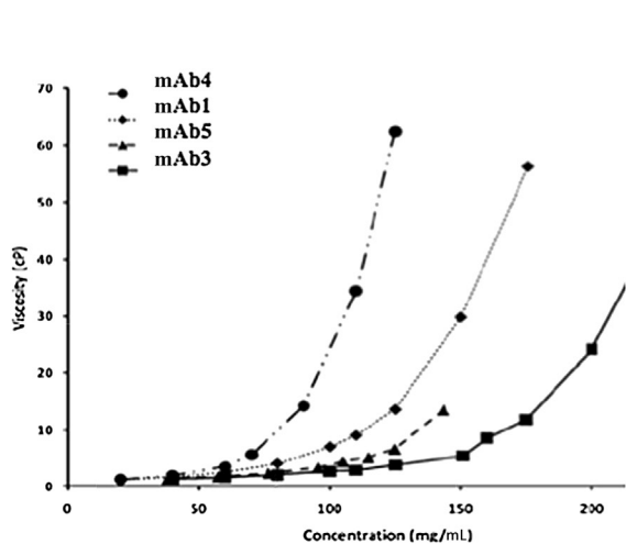
Figure 9.8 Viscosity and net charge for four mAbs at pH 6, 15 mM ionic strength. From Yadav, Laue et al. (2012) .
