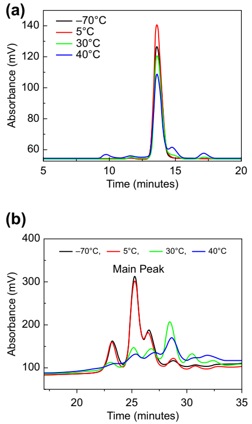
Figure 4.1 Stability of a mAb after 1 year of storage at -70 , 5 , 30 , and 40 °C as assessed by (a) size exclusion chromatography and (b) hydrophobic interaction chromatography after papain digestion. Figure provided by Jun Liu, Genentech.
