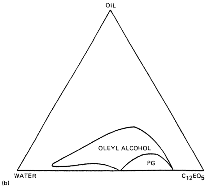
Figure 4.5 (a) Phase diagram at 298 K for the system C_{12}EO_5 -Azone-water. (b) Partial phase diagrams showing the extent of the lamellar phases of the system C_{12}EO_5 -water with oleyl alcohol and propylene glycol at 298 K.
