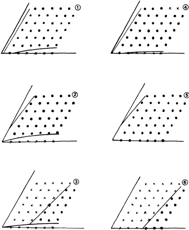
Figure 9.25 Phase behavior results for the ternary systems listed in Table 1 for the hypothetical cream system example. Xs denote either clear single-phase regions, two liquid phases (i.e., an unstable emulsion) or stable emulsion plus another phase.
