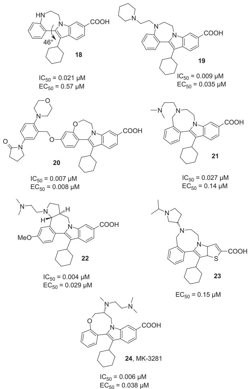
Figure 8.6 Constrained tetracyclic and pentacyclic indole inhibitors from Japan Tobacco and Merck.
