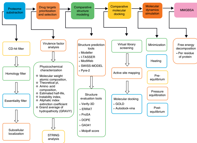
Figure 13.3 A complete step-by-step flow of different methodologies to identify inhibitors of a novel protein target from Acinetobacter baumannii . Source: Reprinted from Ahmad et al. (2018). Copyright (2018), with permission from Elsevier.
