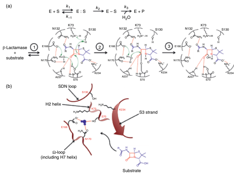
Figure 6.3 Scheme of \beta -lactam antibiotic hydrolysis by \beta -lactamase TEM-1 (a). The structure of the active site of \beta -lactamase TEM-1 with the location of catalytically important residues (b).
