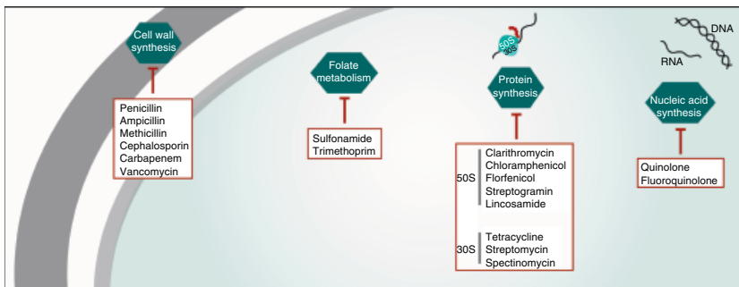
Figure 7.1 Common classes of antibiotic drugs and their targets. Antibiotics relevant for this chapter and their respective targets within a bacterial cell are illustrated.
