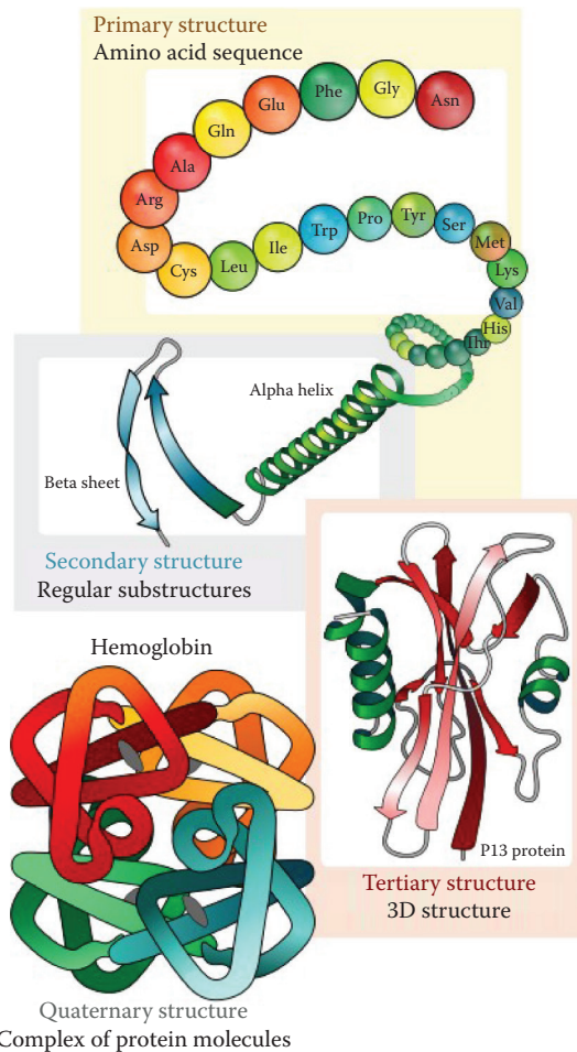
Figure 1.6 The four levels of protein structure.
