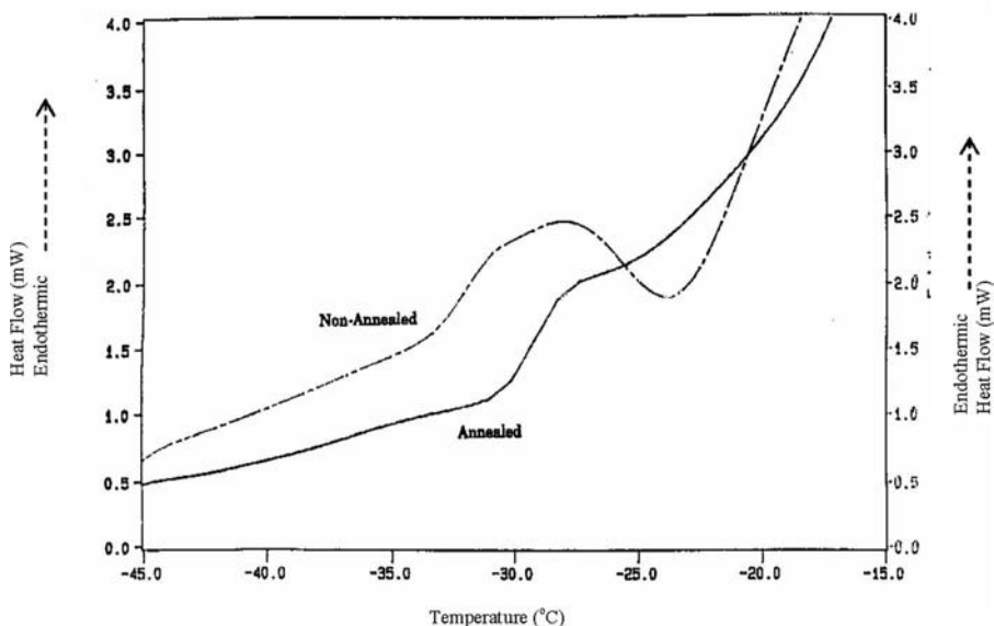
FIGURE 8 Differential scanning calorimetry thermograms for annealed versus non-annealed bulk solution used in CAVERJECT Sterile Powder.
