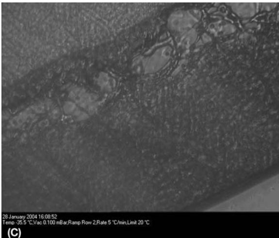
FIGURE 13 Freeze-drying microscopy images on a sample showing (A) frozen, (B) drying, and (C) collapse. Images taken using a 5- \mu L sample on a Linkam FDSC 196 cryostage.
