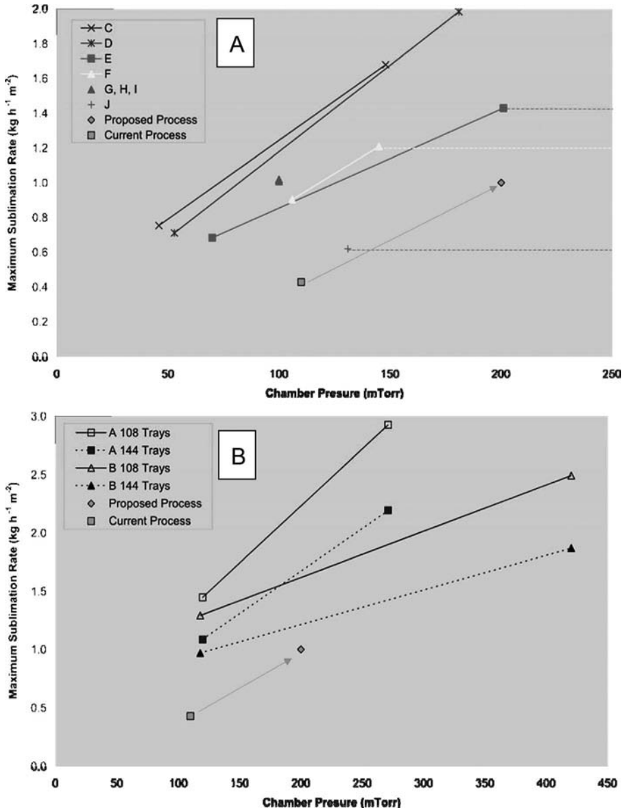
FIGURE 4 Maximum sublimation rate during primary drying, normalized by square meter of shelf space loaded with this product. Combined results from primary drying optimization ( bold black squares and diamonds ) compared to freeze-dryer capabilities. Panel A: Full load in dryers C through J. Panel B: Current partial load (108 trays) as well as full load (144 trays) in freeze-dryers A and B.
