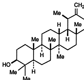
Taraxasterol (97-21)
